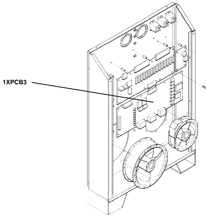
Control Board 1XPCB3
