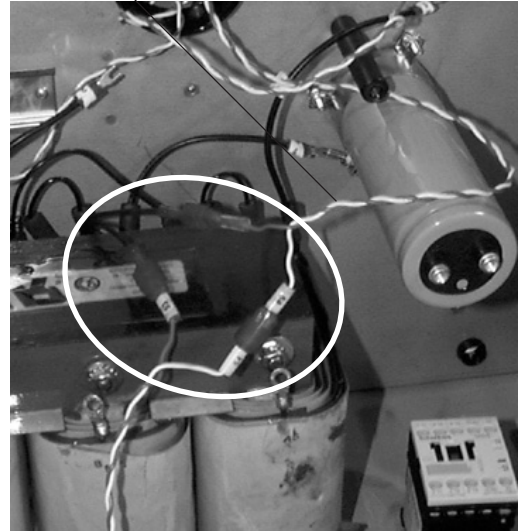
Location of wires in ArcWriter Power Supplies
