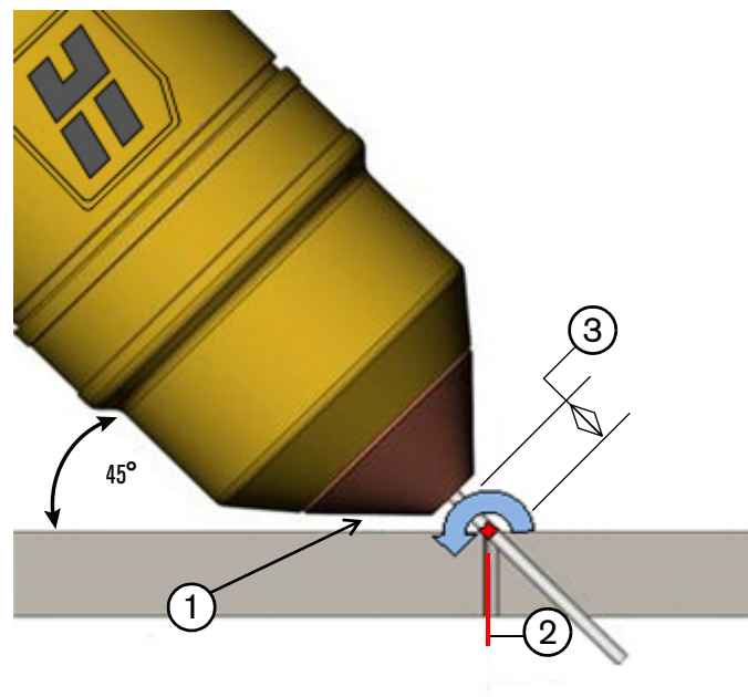
Figure 16 – Elimination of process shift by adding cut height to the bevel pivot length
