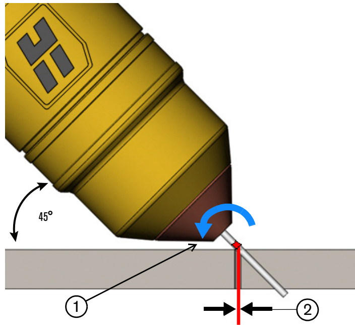
Figure 13 – Impact of the TPL on process shift when TPL = 2.358 inches (59.89 mm)
