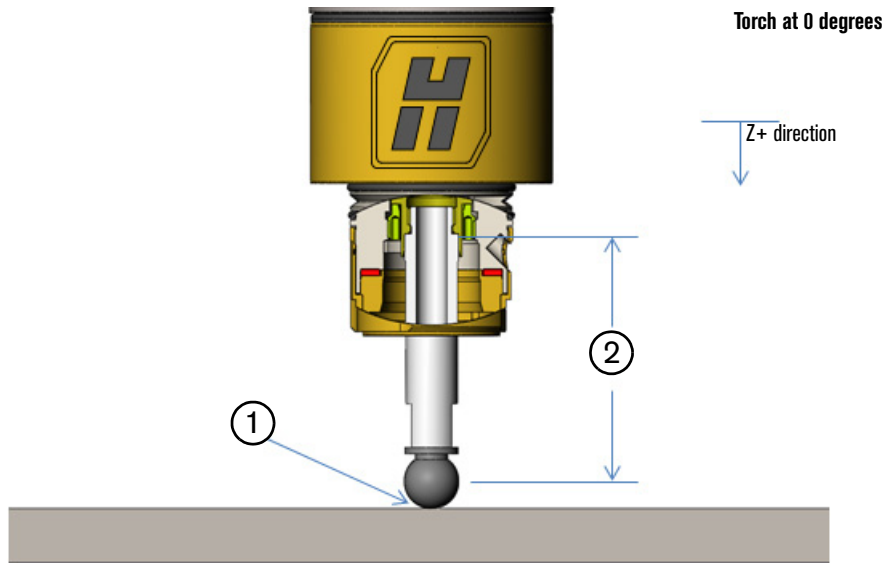
Figure 18 – Example of using a bevel head alignment tool for determining Z_0 .
