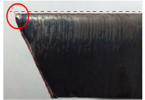
Figure 6 – A cut part size reduction due to top corner rounding
