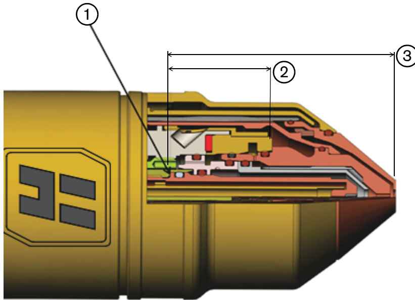
Figure 10 – Example of the TPL for the bevel pivot point located at the tip of a 130 A shield
