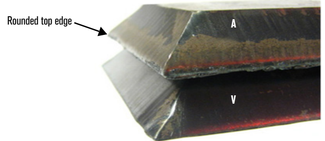
Figure 5 – V cut–A cut edge comparison
