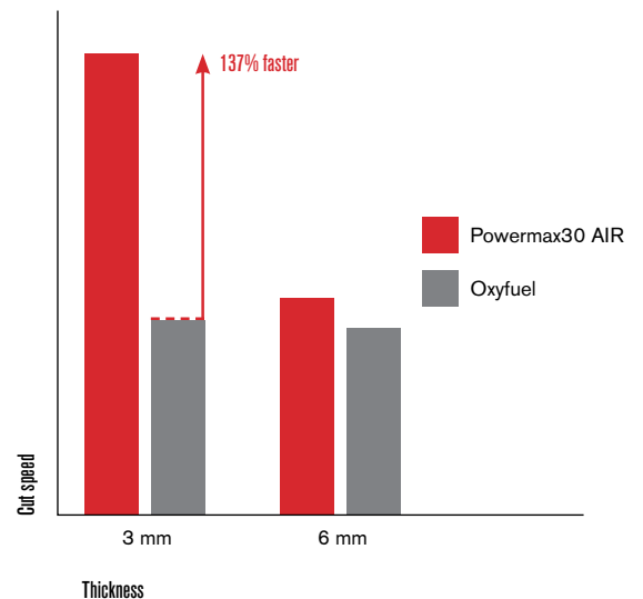
Relative cut performance on mild steel
