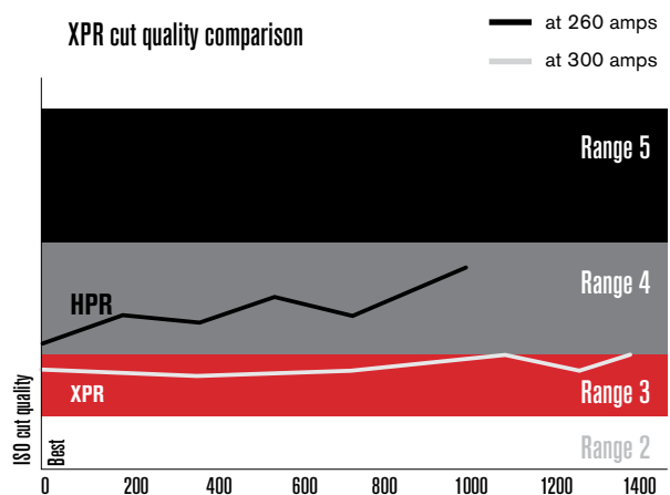
20-second cuts on 20 mm (3/4") mild steel
