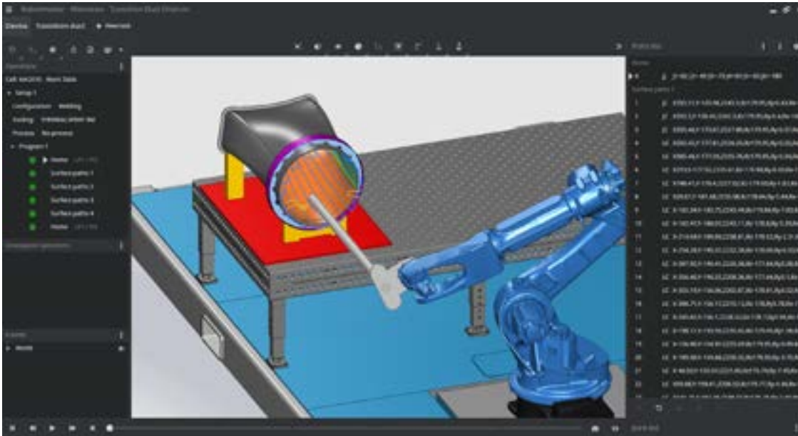
Robotmaster used to program a Motoman robot to perform thermal spraying on a transition duct.
